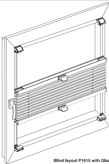
Blind layout P1615 with Glazing Bead Mounts
